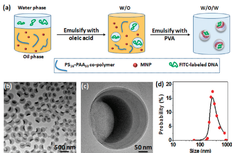
Figure 1. Nanocapsule synthesis and size characterization. (a) Schematic illustration of the key steps in nanocapsule preparation. In the first step (W/O emulsion), an aqueous solution of hydrophilic compounds ( e.g. , biologics) is emulsified in a volatile organic solvent (in this paper, chloroform) with oleic acid as the surfactant, followed by the second round emulsion (W/O/W) with PVA as the surfactant. (b,c) TEM images of the nanocapsules prepared via the double emulsion approach. The scale bars are 500 nm for the low-magnification image, and 50 nm for the high-magnification image. (d) Hydrodynamic size (263 ± 42 nm) of the nanocapsules measured by DLS.
